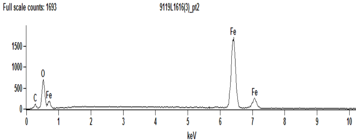
Figure 13. SEM-EDS spectrum from Spot 2 on the gray layer (bottom) in Figure 11.
