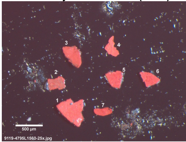
Example of the red/gray chips mounted on a carbon tab. Sample L1560 - Murray & Church St.
