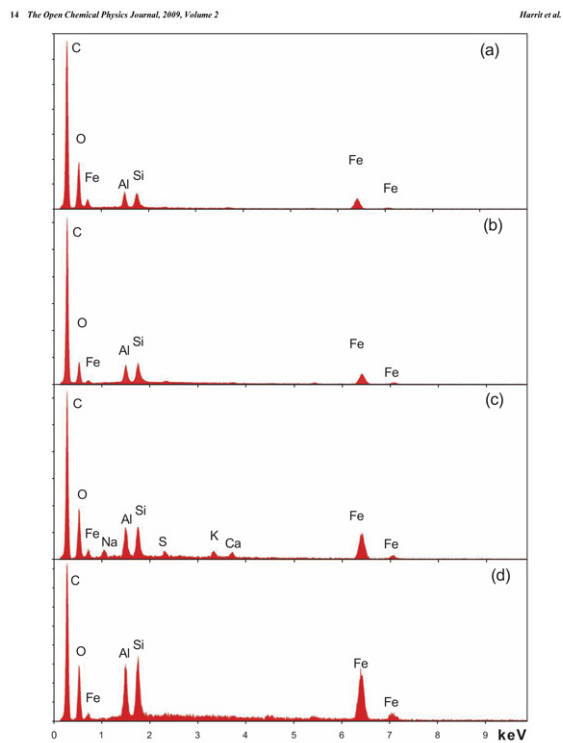
Fig. (7). XEDS spectra obtained from the red layers from each of the four WTC dust samples, with (a) corresponding to sample 1 and so on (b-d).
