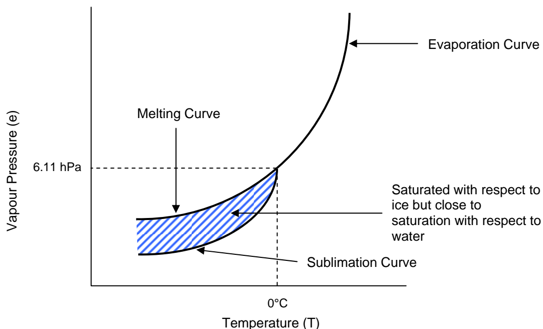
Figure 8. There is a maximum amount of water vapour the air, at a given temperature, can hold.
