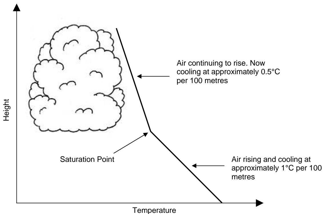
Figure 9. Temperature profile of a parcel of air as it rises through the atmosphere.
